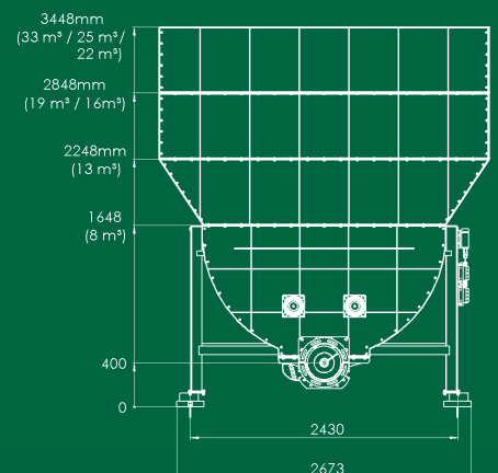
SBCV-19 cbm Four-way attachment
